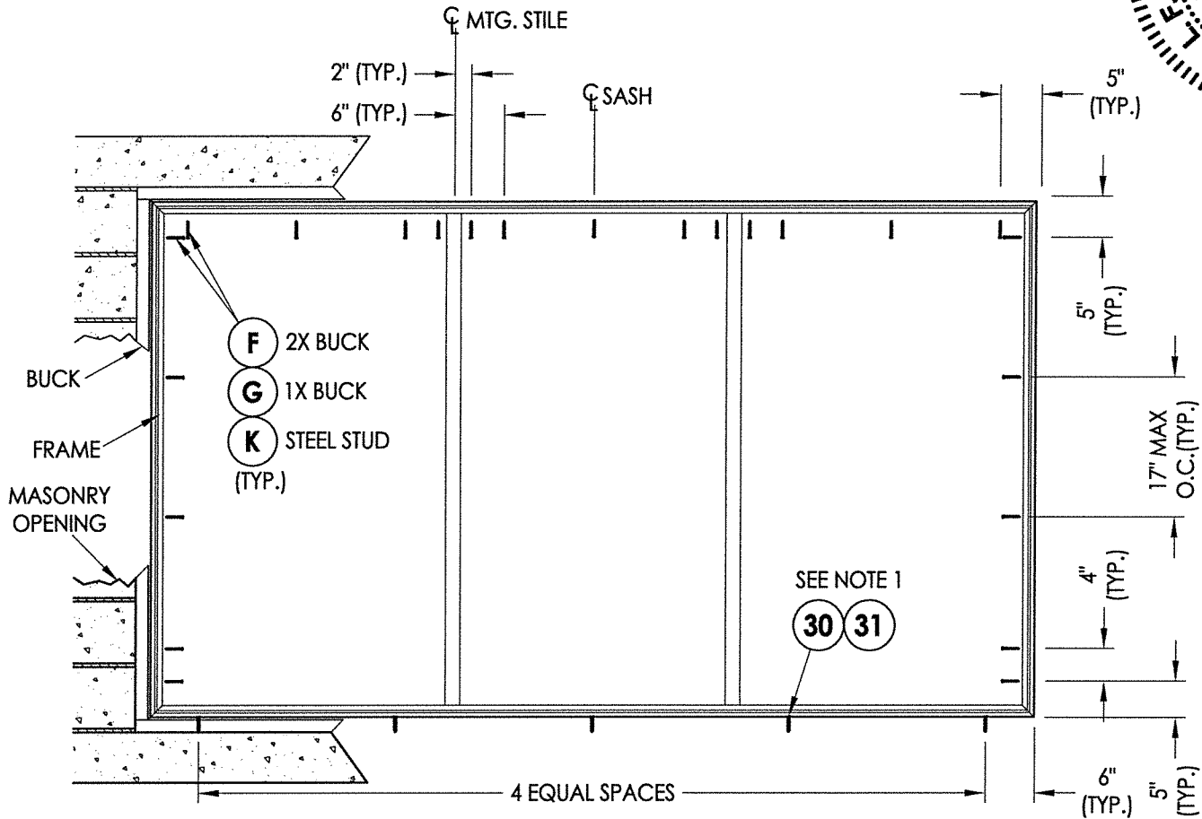
FRAME ANCHORING
