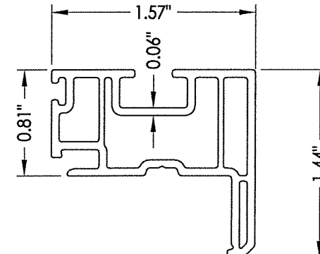
5 TOP RAIL
