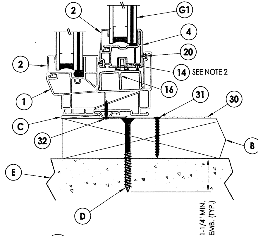
3 2 VERTICAL CROSS SECTION 2X Buck Masonry Construction
