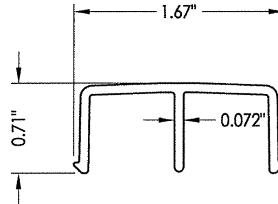
16 ROLLER TRACK
