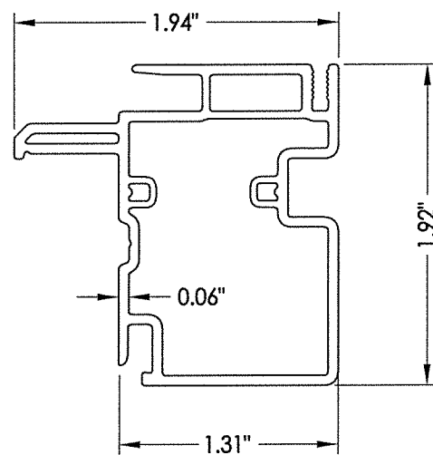
6 MEETING STILE
