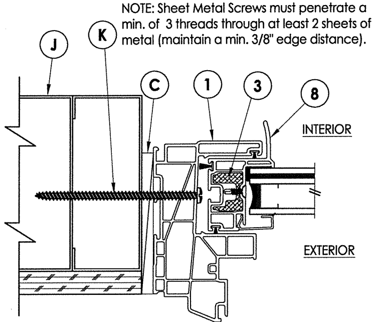
4 2 HORIZONTAL CROSS SECTION Metal Stud Construction
